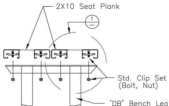
SIDE VIEW OF BENCH ASSEMBLY
