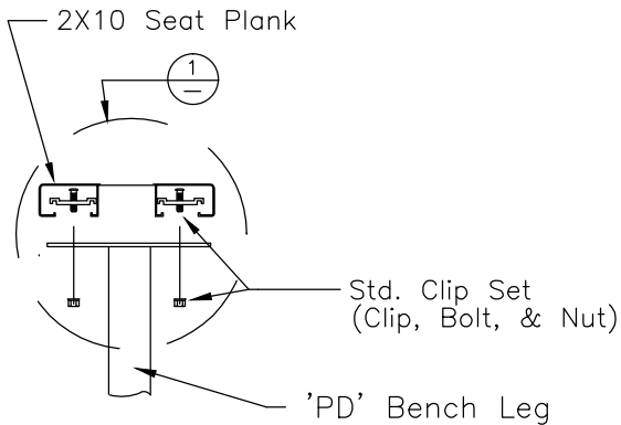
SIDE VIEW OF BENCH ASSEMBLY
