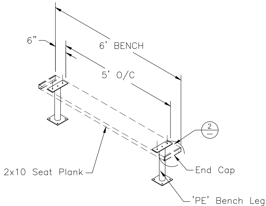
ISOMETRIC VIEW OF BENCH ASSEMBLY
