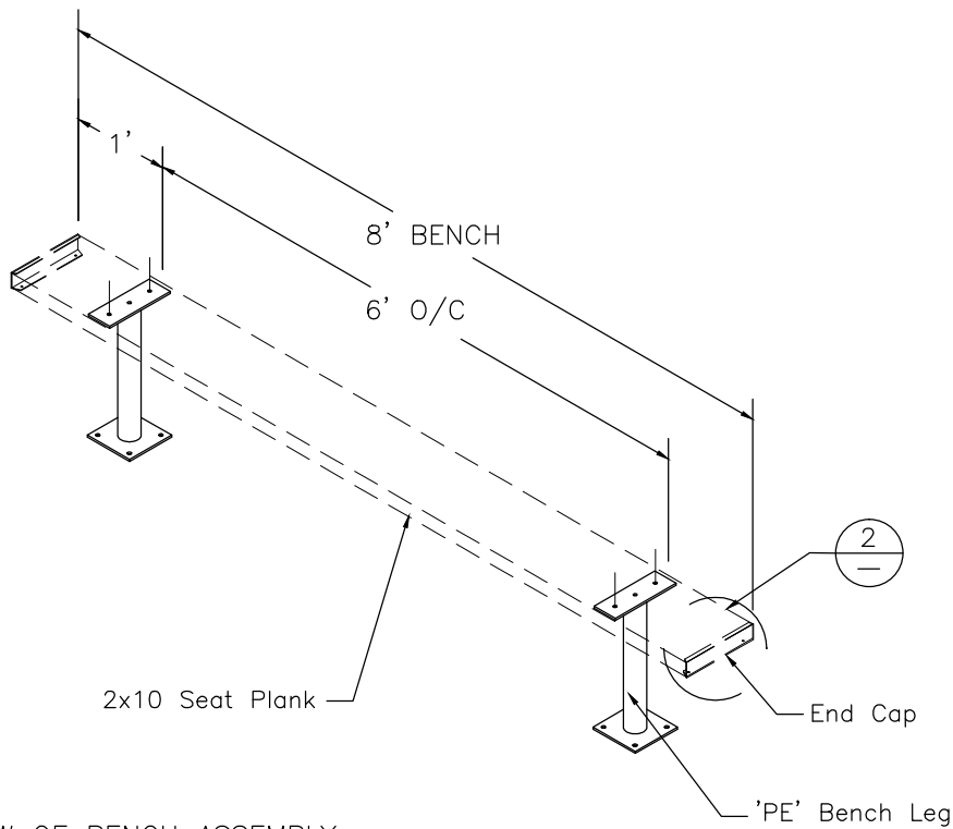
ISOMETRIC VIEW OF BENCH ASSEMBLY
